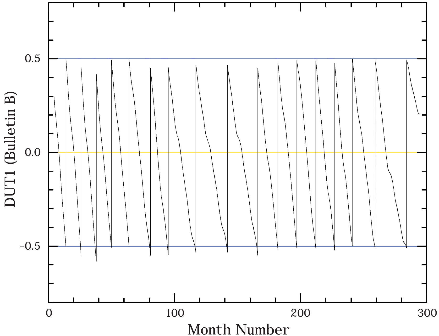
Figure 4: Monthly Leap Second Scheduling
